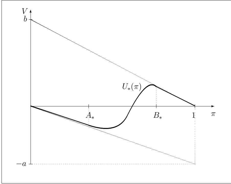
Figure 1. A computer drawing of the reference (difference) function \pi \mapsto U_*(\pi) on [0, 1] .
